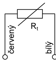
two - wire
